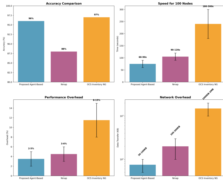
Fig. 7: Performance Evaluation of Proposed approach, Nmap and OCS Inventory NG
