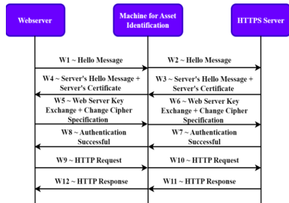
Fig. 1: Example of SSL Spoofing for Fingerprinting of Web Server
