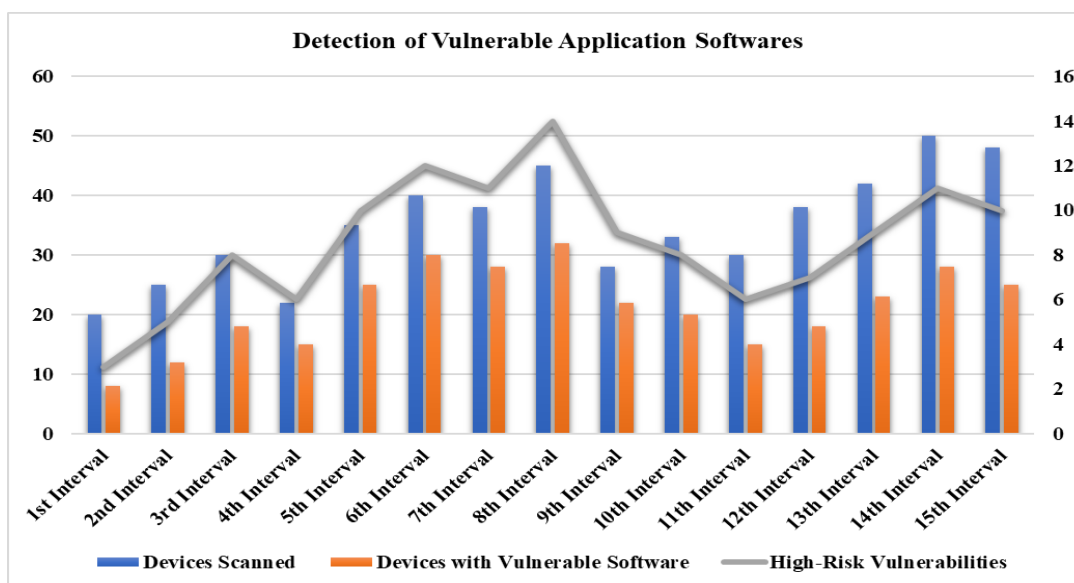
Fig. 6: Comparative Analysis of Detection of Vulnerable Application Software in Campus Area Network (15 Intervals)
