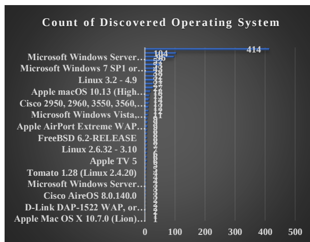
Fig. 3: Count of Discovered Operating System with Nmap Network Discovery Tool
